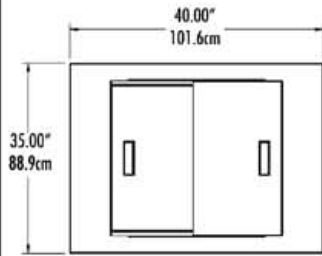
Plan View SPH-40EW
