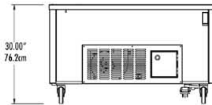
Elevation View SPH-50EW
