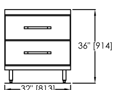
Model C11043-32 Increases standard 24" refrigerated section 8" to 32" - 29" or 33" deep bases. Supplied with (2) 12" x 20" x 6" dp. plastic pans per drawer.
