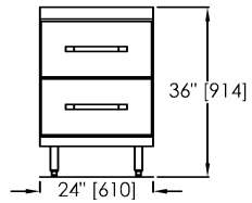
Model C11043-24 Fits standard 24" refrigerated sections. Available in 29" or 33" deep bases. 33" deep model supplied with (1) 12" x 20" x 6" dp. plastic pan per drawer.
