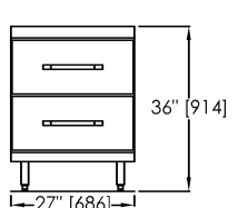
Model C11043-27 Increases standard 24" refrigerated section 3" to 27". - 29" or 33" deep bases. Supplied with (2) 12" x 20" x 6" dp. plastic pans per drawer.
