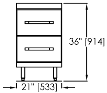
Model C11043-21 Fits standard 21" refrigerated sections. Available in 29" or 33" deep bases. 33" deep model supplied with (1) 12" x 20" x 6" dp. plastic pan per drawer.
