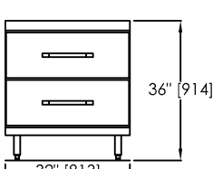
Model C11043-32E Increases standard 24" refrigerated section 8" to 32" - 29" or 33" deep bases. Supplied with (2) 12" x 20" x 6" dp. plastic pans per drawer.
