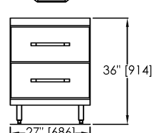
Model C11043-27E Increases standard 24" refrigerated section 3" to 27" - 33" deep bases only . Supplied with (2) 12" x 20" x 6" dp. plastic pans per drawer.
