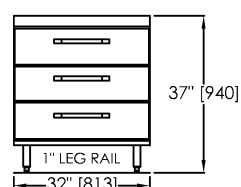
Model C11043-32TE Increases standard 24" refrigerated section 8" to 32" - 29" or 33" deep bases. Supplied with (2) 12" x 20" x 4" dp. plastic pans per drawer.
