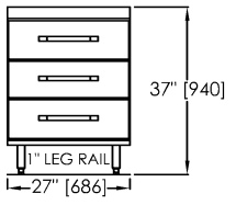
Model C11043-27TE Increases standard 24" refrigerated section 3" to 27" - 33" deep bases only . Supplied with (2) 12" x 20" x 4" dp. plastic pans per drawer.
